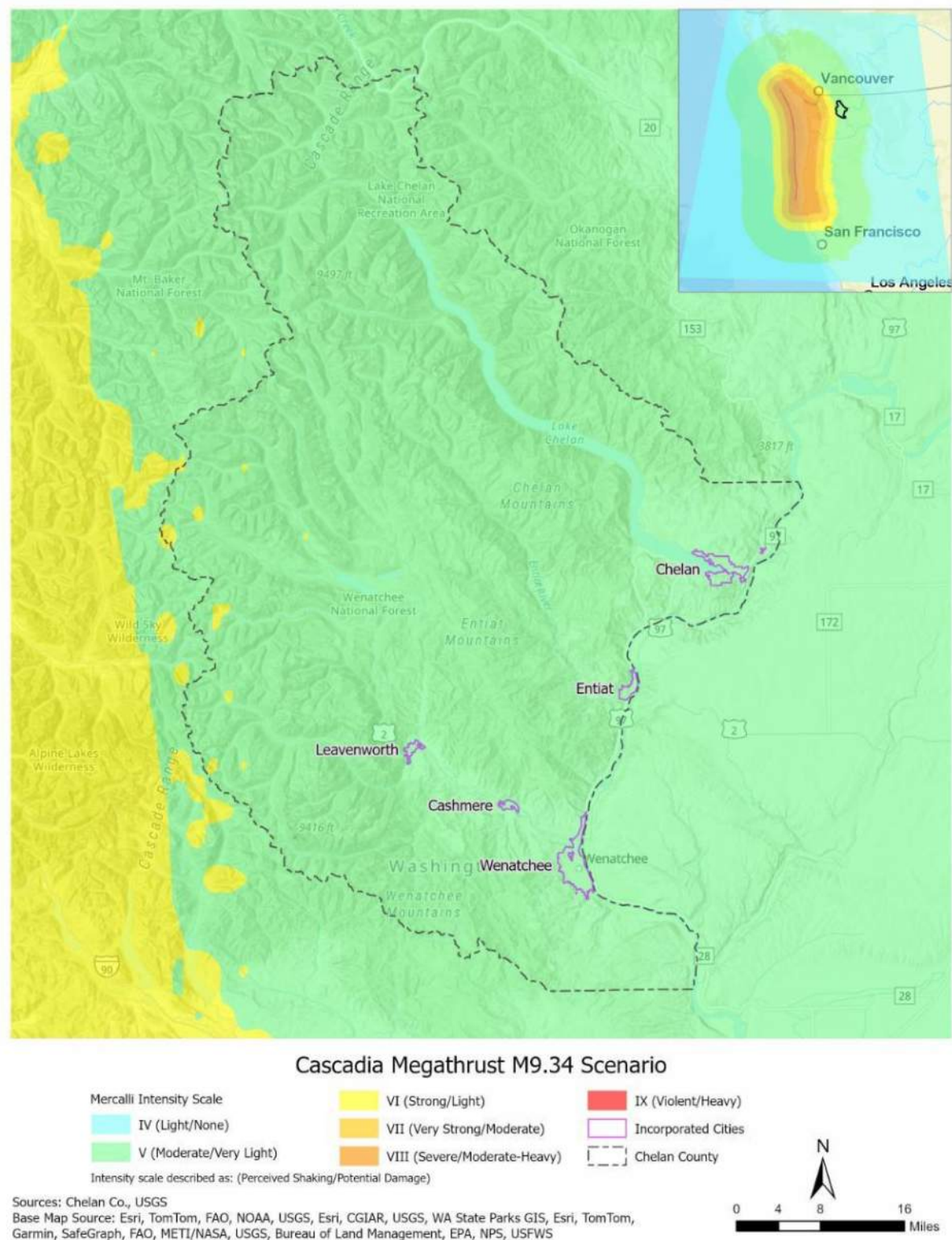
Figure 11-9. Cascadia M9.0 ShakeMap Scenario
